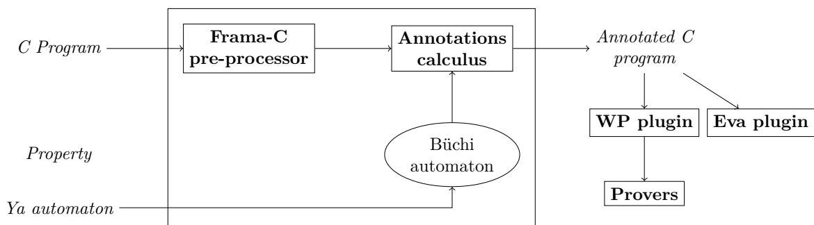
Figure 5.2: Plug-in Structure
