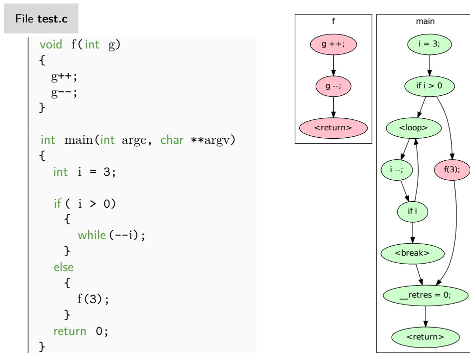
Figure 2.3: Control flow graph colored with reachability information.
