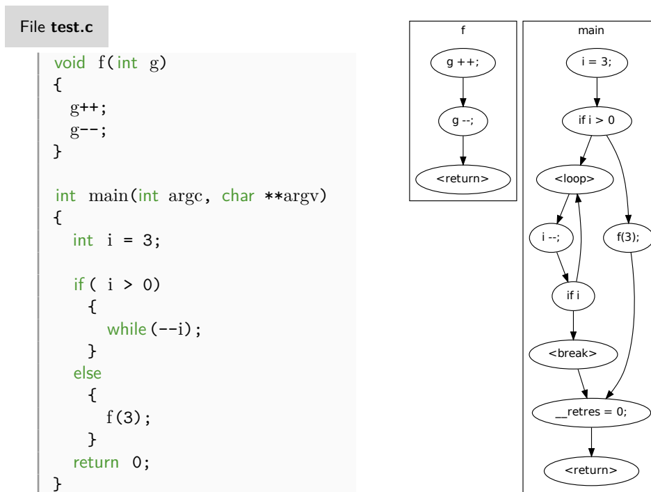
Figure 2.2: Control flow graph for file test.c .
